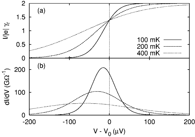
FIG. 11. Dependence of (a) the current step and (b) the conductance peak on the temperature in the two-levels-accessible case in the presence of nonequilibrium. We assume \gamma'_1 = \gamma'_2 = \gamma_l and \gamma'_1 = \gamma'_2 = \gamma_r , with \gamma_l \gg \gamma_r and no relaxation in the island.
